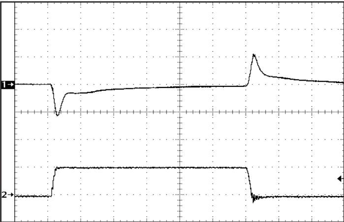
Figure 12: Output voltage response to step-change in load current (0%-50%- 0% of Iout (max)). Load cap: 1μ F ceramic cap and 10μ F, 100 mW ESR tantalum cap. Ch 1: Vout (300mV/div). Ch 2: Iout (10A/div).
