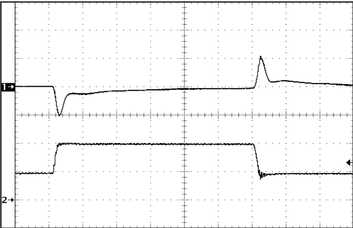
Figure 11: Output voltage response to step-change in load current (50%-100%-50% of Iout (max)). Load cap: 1μ F ceramic cap and 10μ F, 100 mW ESR tantalum cap. Ch 1: Vout (300mV/div). Ch 2: Iout (10A/div).
